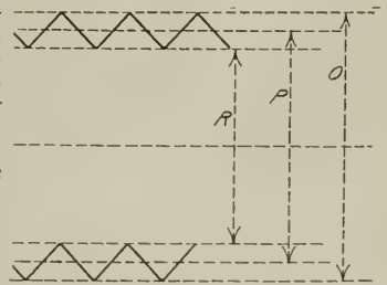
O = Outside diameter P = Pitch diameter R = Root diameter FIG. 3.
